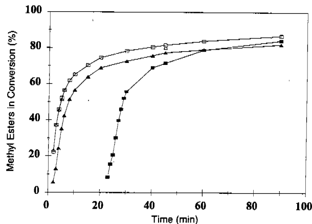
FIG. 2. The effect of mixing intensity and time on the overall conversion to methyl esters at 50°C. ( \blacksquare ) N_{Re} = 3100; ( \blacktriangle ) N_{Re} = 6200; ( \square ) N_{Re} = 12400; ( \triangle ) N_{Re} = 18600. See Figure 1 for abbreviation.
