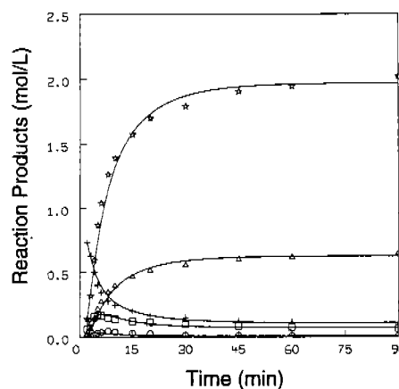
FIG. 5. Kinetic modeling curves and experimental points for the composition of the reaction mixture during the transesterification of soybean oil at 50°C and N_{Re} = 6200 . (+) Triglycerol; (☆) methyl esters; (□) diglycerides; (○) monoglycerides; (△) glycerol. See Figure 1 for abbreviation.
