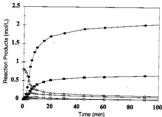
FIG. 1. The composition of the reaction mixture during the transesterification of soybean oil at 50°C and Reynolds number ( N_{Re} ) = 6200. ( \Delta ) triglycerides; ( \bullet ) methyl esters; (X) diglycerides; ( \square ) monoglycerides; ( \blacksquare ) glycerol.
