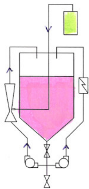
Inject and mix Acid
