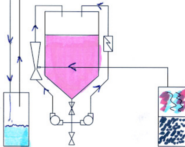
Recover, Heat, and mix Methanol into new oil while recovering Methanol from glycerin
