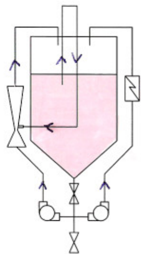
Mix reactor "top layer" contents with bottom during mix cycles.
