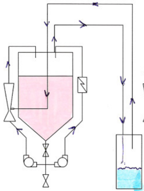
Recover Methanol from Biodiesel
