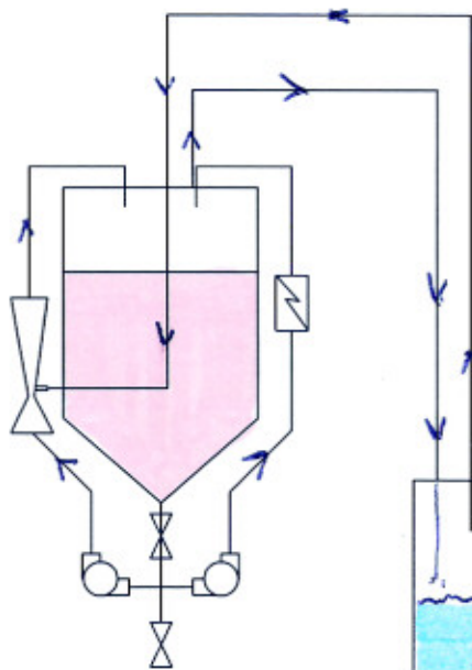
Recover Methanol from Biodiesel
