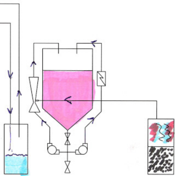
Recover, Heat, and mix Methanol into new oil while recovering Methanol from glycerin
