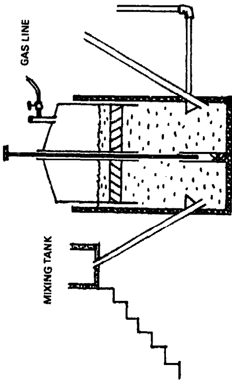
FIG. 19-1 STA. BARBARA BIOGAS PLANT (MAYA FARMS-INDIA)
